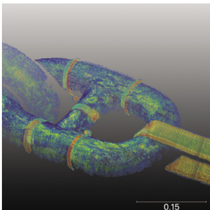
High resolution 3D scan of a marine anchor chain showing corrosion in full color (Source: Kraken Robotics)
