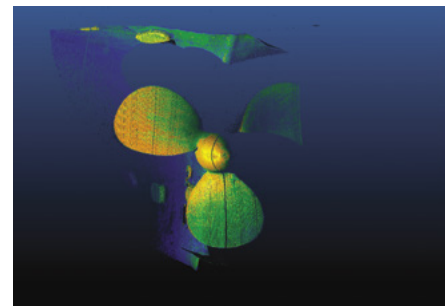
3D underwater inspection of a three-blade propeller with millimeter accuracy (Source: Kraken Robotics)
