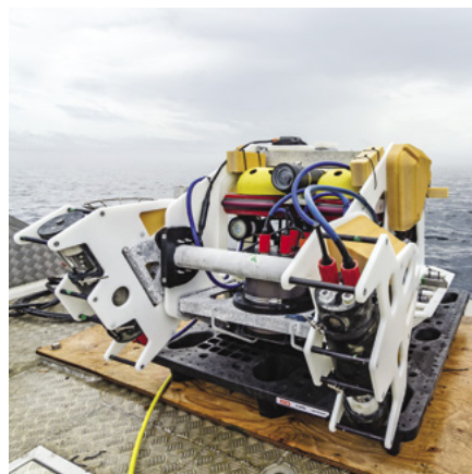
SeaVision ™ mounted on unmanned underwater vehicle (Source: Kraken Robotics)
