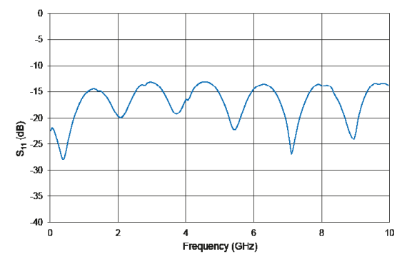
MX-LN-05 Typical S_{11} Curve
