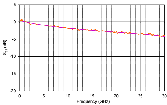
MX-LN-40 Typical S_{21} Curve
