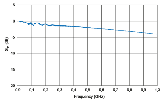
MX-LN-0.1 Typical S_{11} Curve
