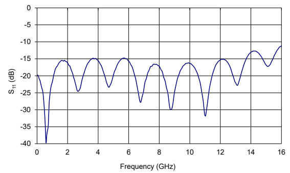
MX-LN-20 Typical S_{11} Curve
