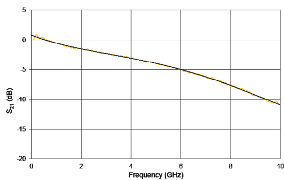
MX-LN-05 Typical S_{21} Curve
