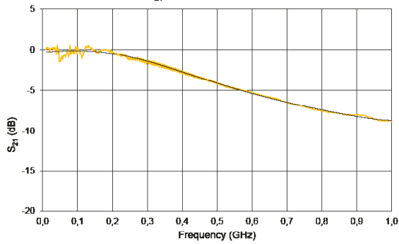
MX-LN-0.1 Typical S_{21} Curve
