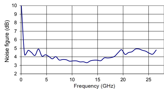
Noise Figure Curve
